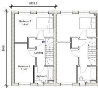
06 First Floor Plan 1 : 100
